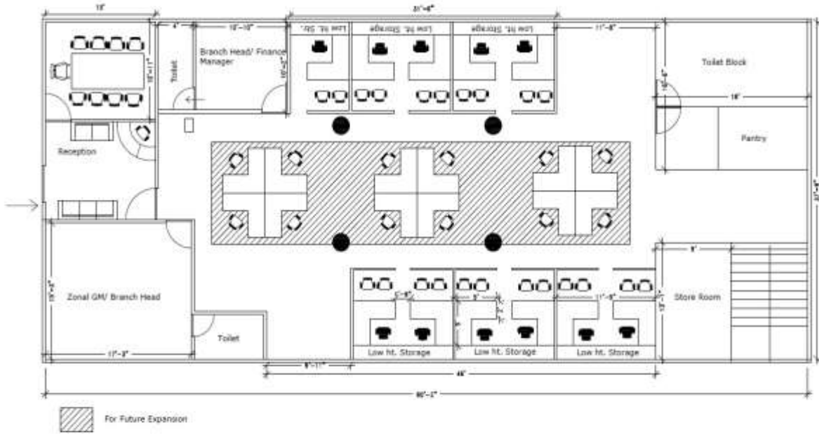
Proposed Layout Plan of Navi Mumbai Office
